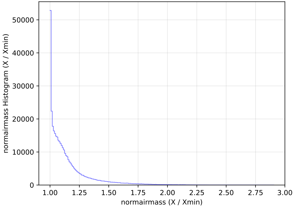
internal_u_expt45_nscale0.9v3.4_10yrs All sky y band: normairmass Histogram
