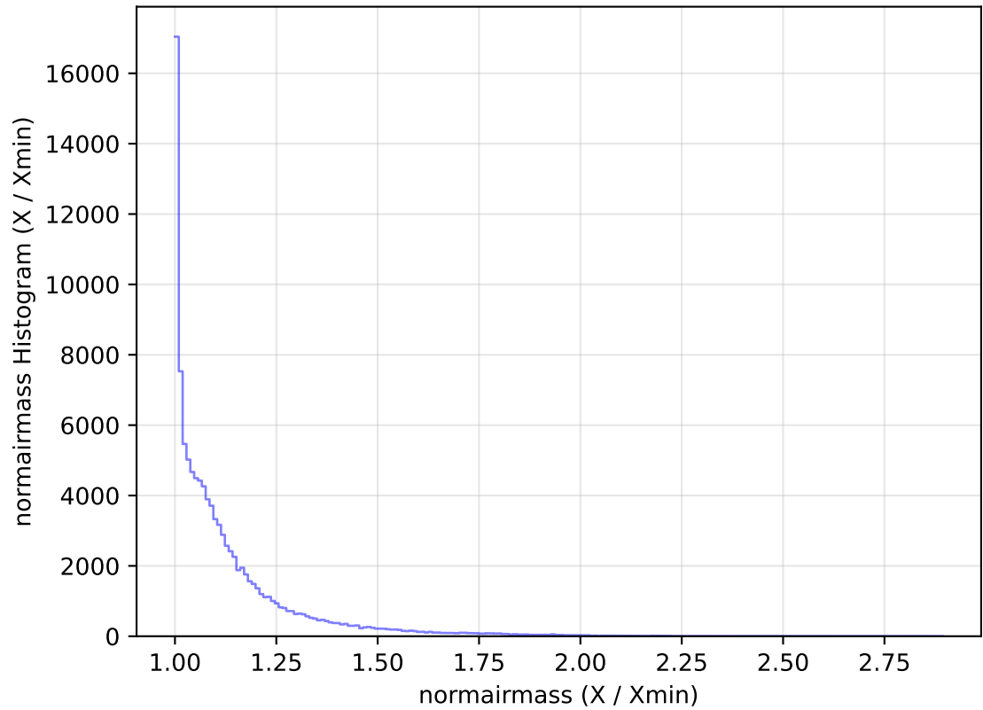
internal_u_expt45_nscale0.9v3.4_10yrs All sky u band: normairmass Histogram
