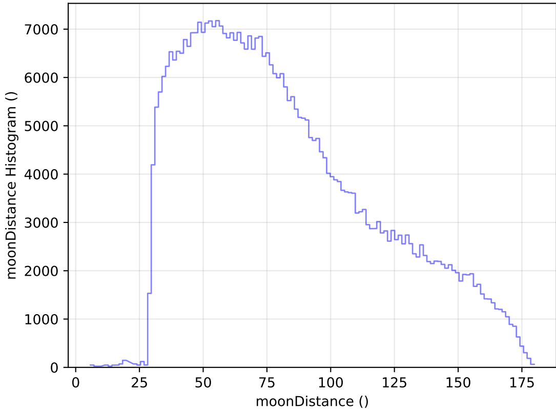
internal_u_expt45_nscale0.9v3.4_10yrs WFD z band: moonDistance Histogram
