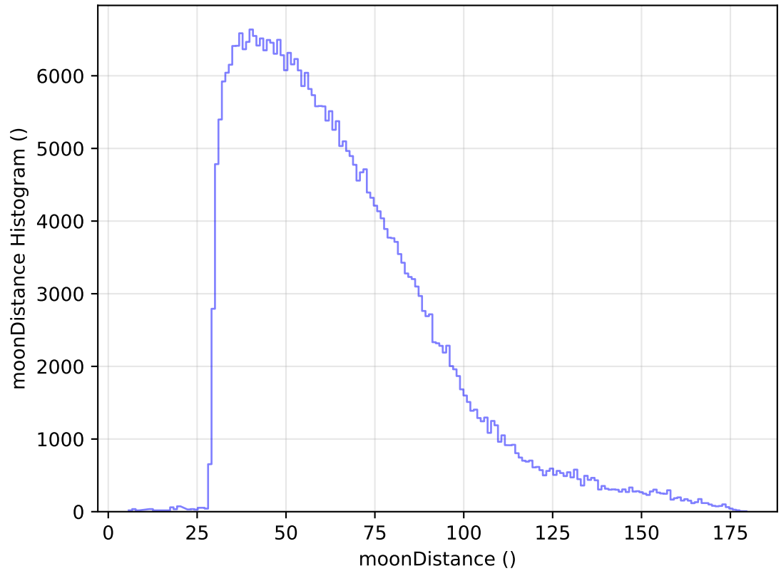
internal_u_expt45_nscale0.9v3.4_10yrs WFD y band: moonDistance Histogram
