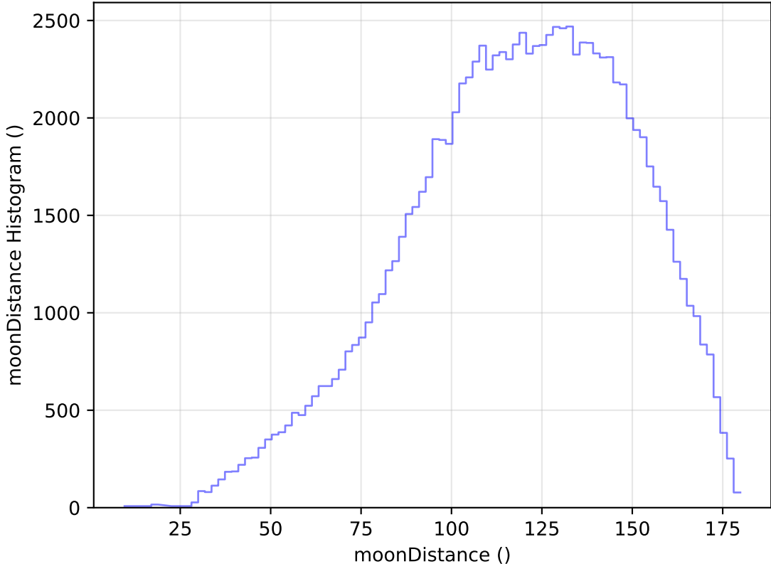
internal_u_expt45_nscale0.9v3.4_10yrs WFD u band: moonDistance Histogram
