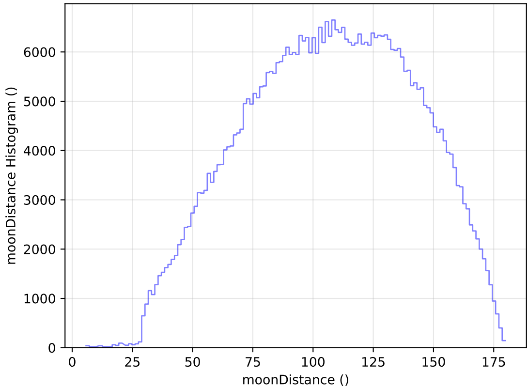
internal_u_expt45_nscale0.9v3.4_10yrs WFD r band: moonDistance Histogram
