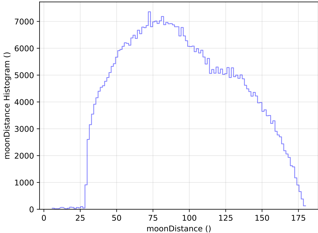
internal_u_expt45_nscale0.9v3.4_10yrs WFD i band: moonDistance Histogram
