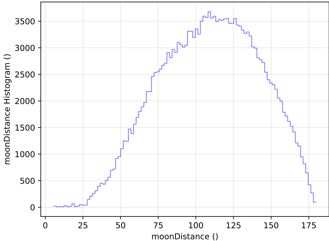
internal_u_expt45_nscale0.9v3.4_10yrs WFD g band: moonDistance Histogram
