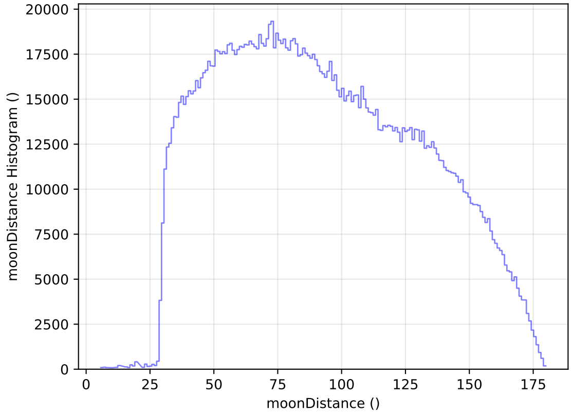
internal_u_expt45_nscale0.9v3.4_10yrs WFD all bands: moonDistance Histogram
