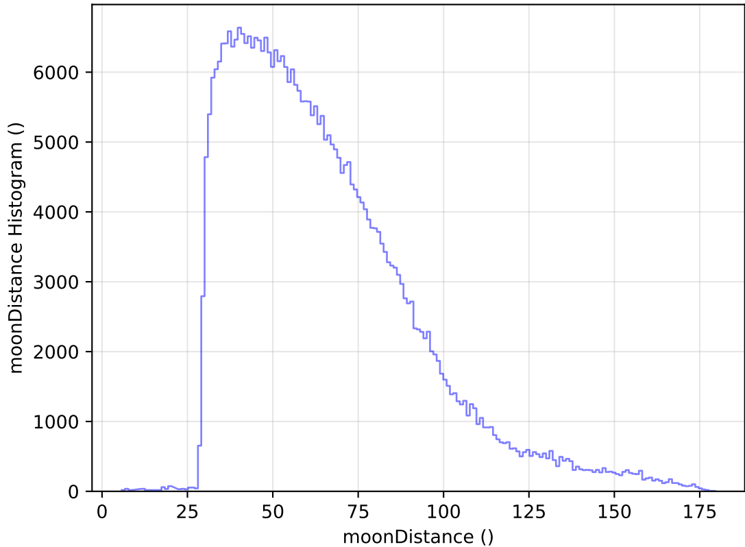
internal_u_expt45_nscale0.9v3.4_10yrs All sky y band: moonDistance Histogram
