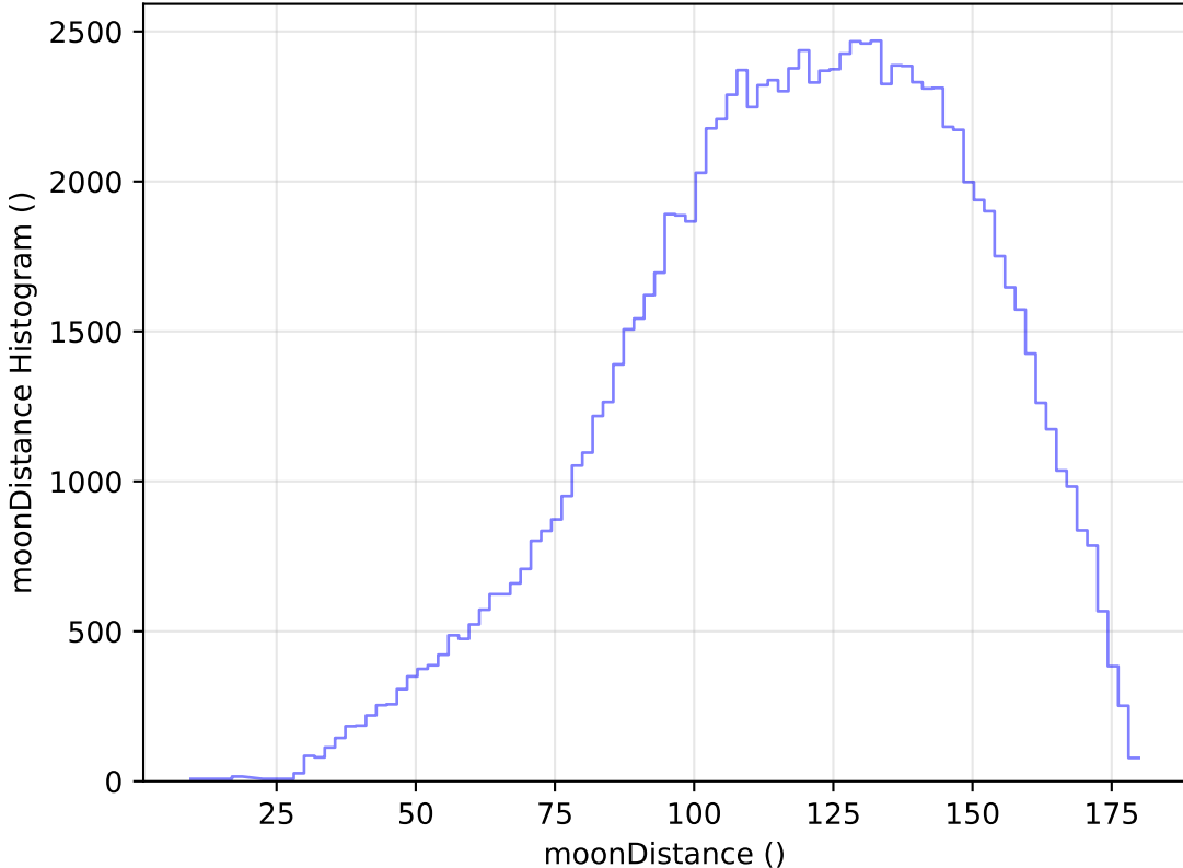
internal_u_expt45_nscale0.9v3.4_10yrs All sky u band: moonDistance Histogram
