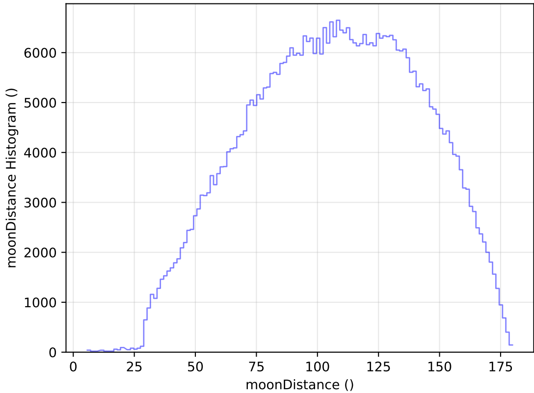
internal_u_expt45_nscale0.9v3.4_10yrs All sky r band: moonDistance Histogram
