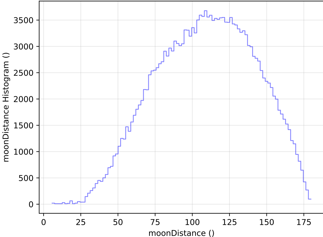
internal_u_expt45_nscale0.9v3.4_10yrs All sky g band: moonDistance Histogram
