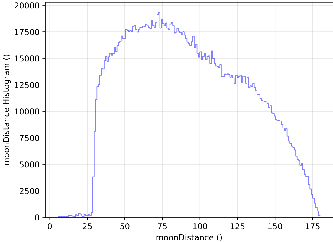
internal_u_expt45_nscale0.9v3.4_10yrs All sky all bands: moonDistance Histogram
