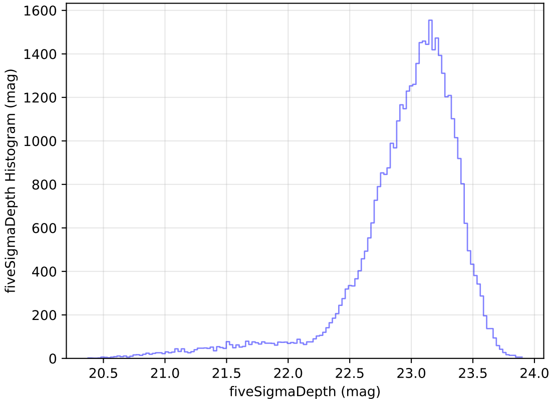
internal_u_expt45_nscale0.9v3.4_10yrs Yr 1 z band: fiveSigmaDepth Histogram
