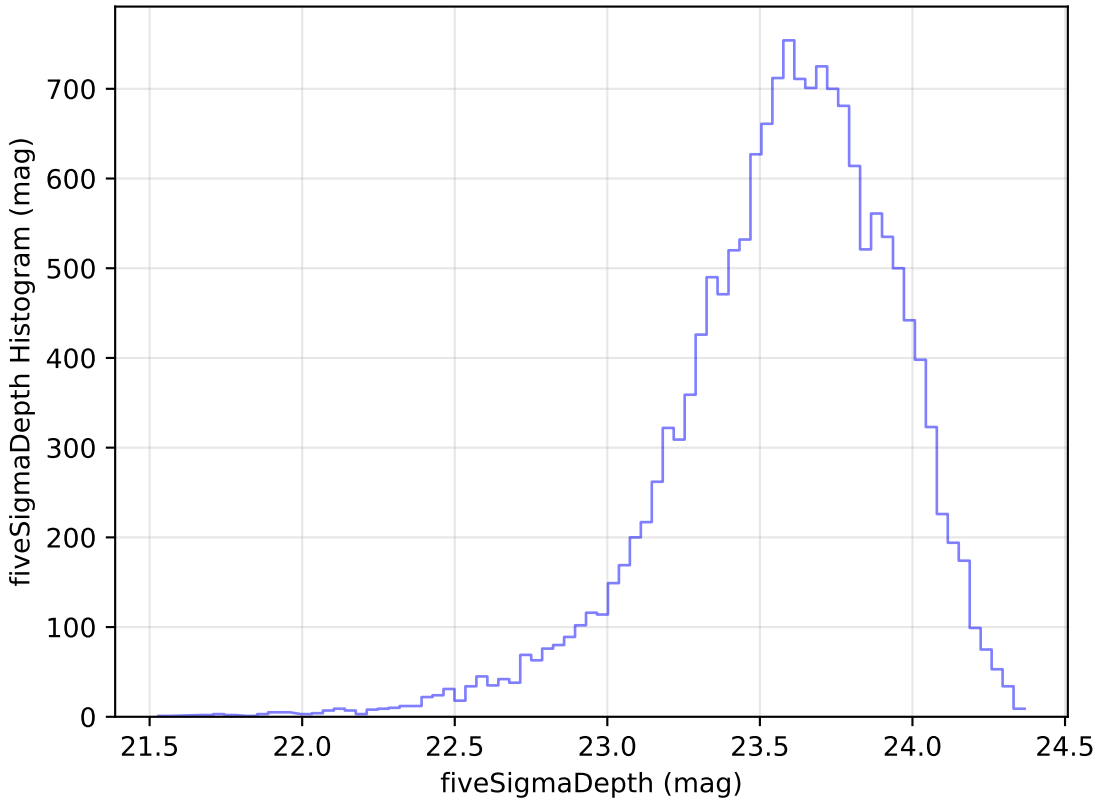
internal_u_expt45_nscale0.9v3.4_10yrs Yr 1 u band: fiveSigmaDepth Histogram
