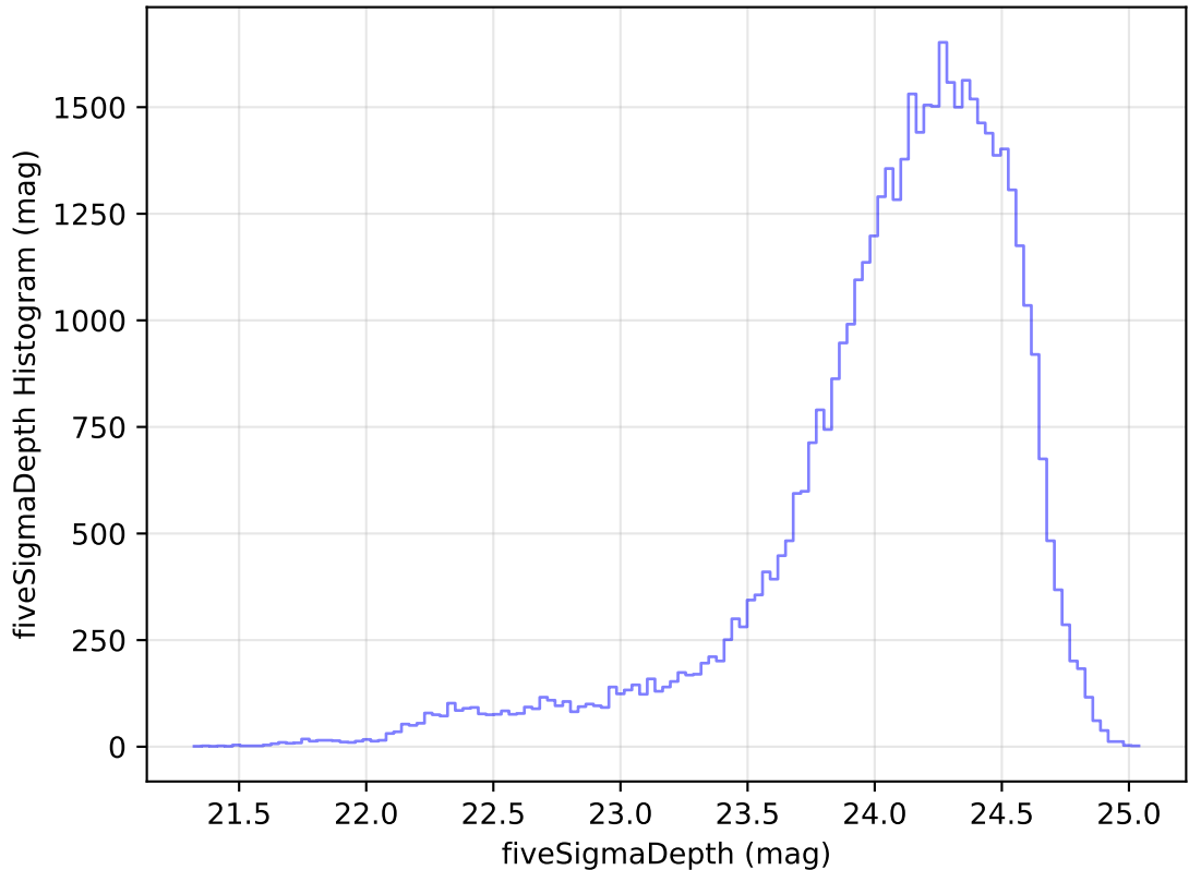
internal_u_expt45_nscale0.9v3.4_10yrs Yr 1 r band: fiveSigmaDepth Histogram
