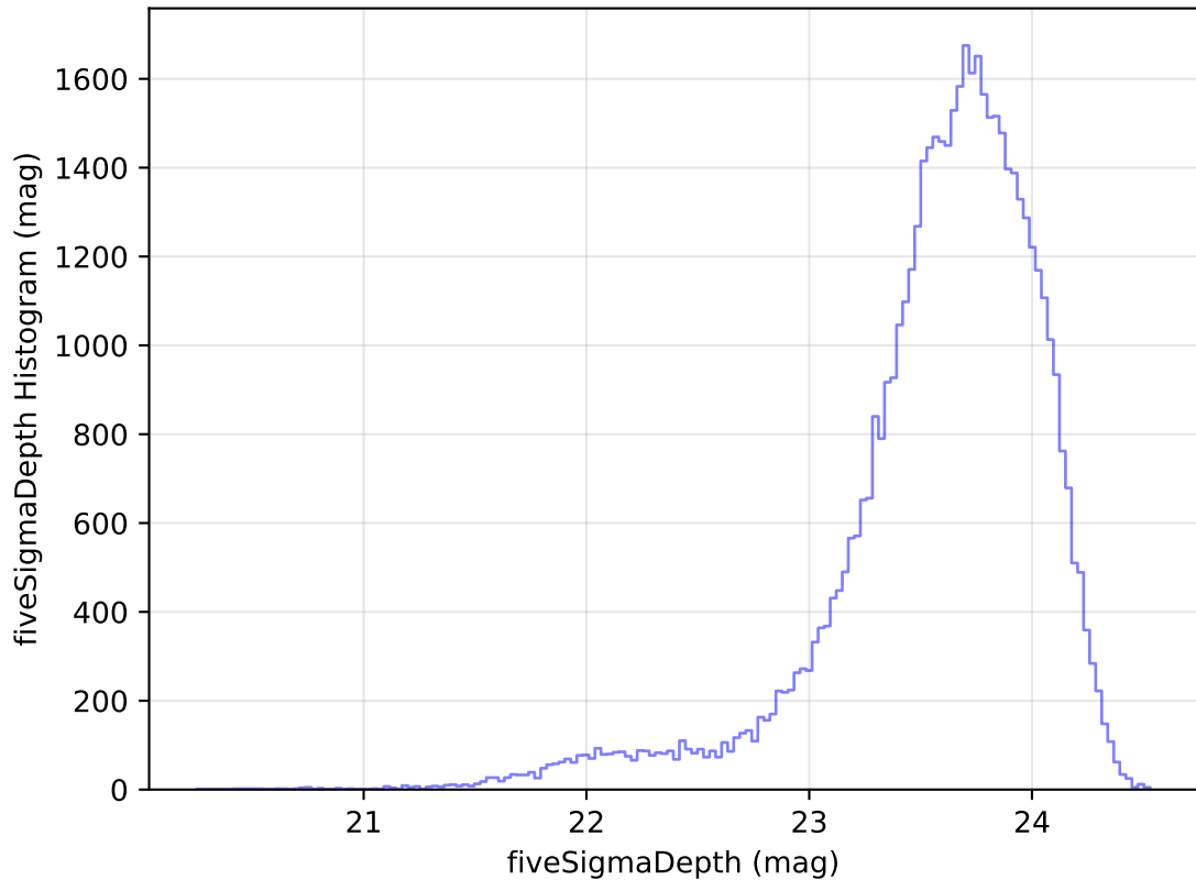
internal_u_expt45_nscale0.9v3.4_10yrs Yr 1 i band: fiveSigmaDepth Histogram
