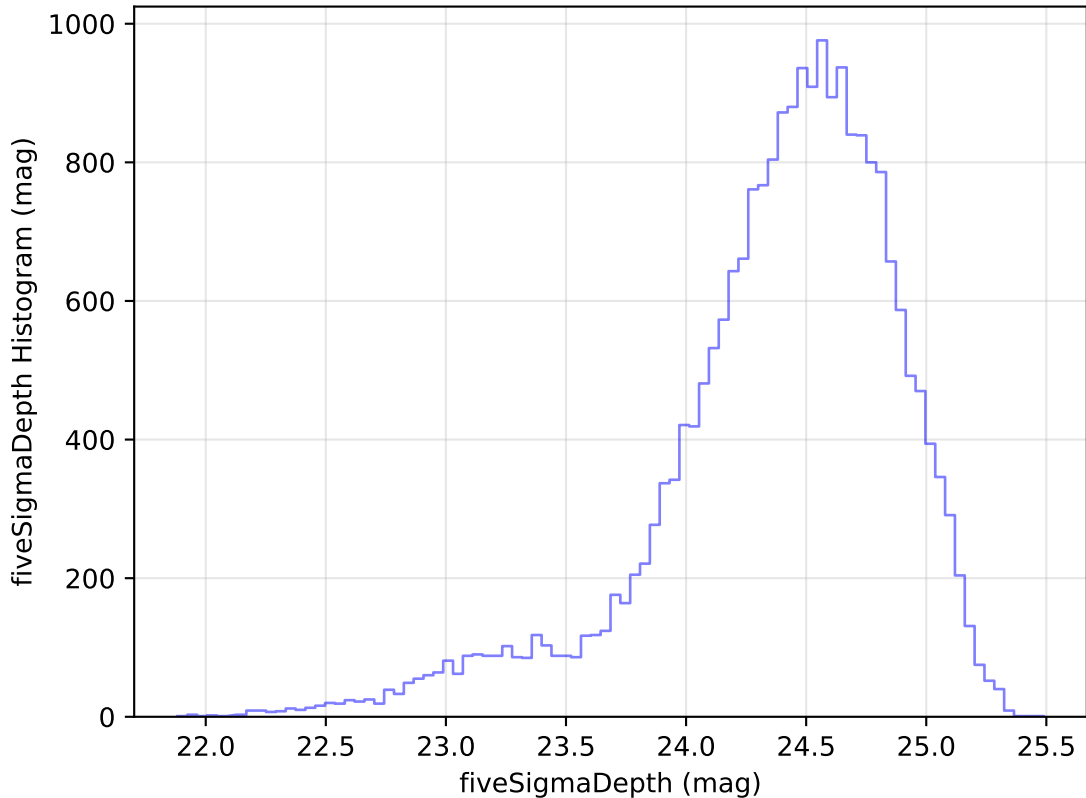
internal_u_expt45_nscale0.9v3.4_10yrs Yr 1 g band: fiveSigmaDepth Histogram
