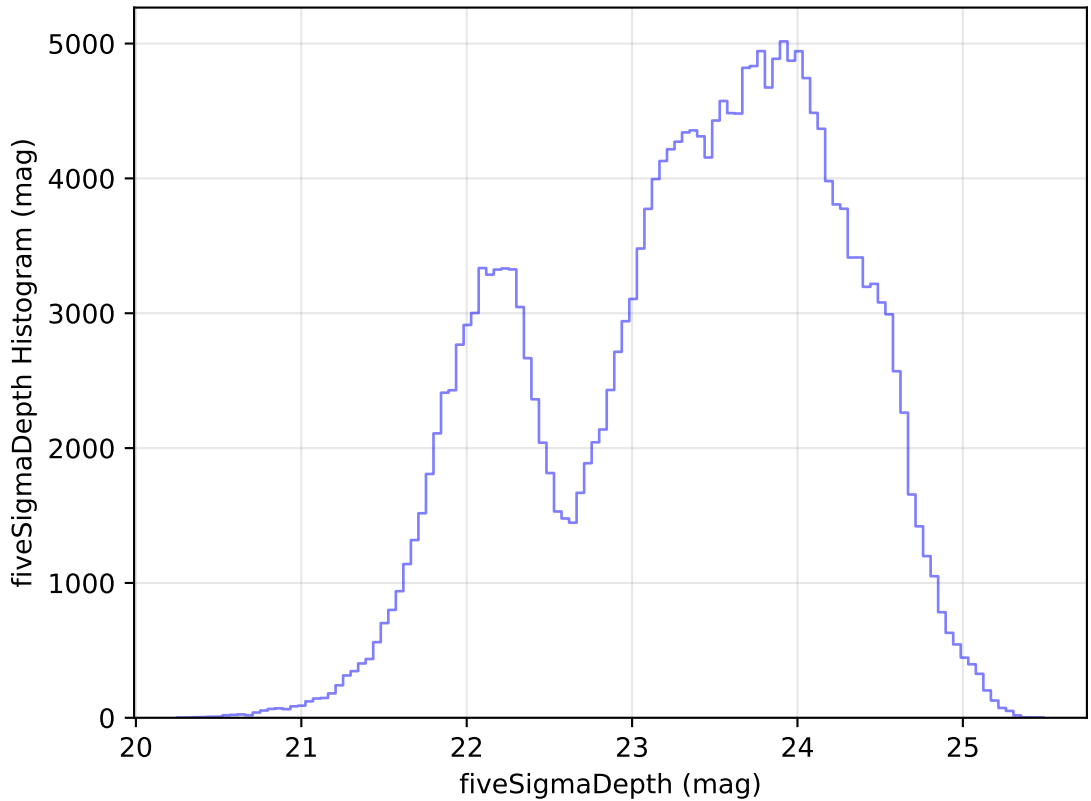
internal_u_expt45_nscale0.9v3.4_10yrs Yr 1 all bands: fiveSigmaDepth Histogram
