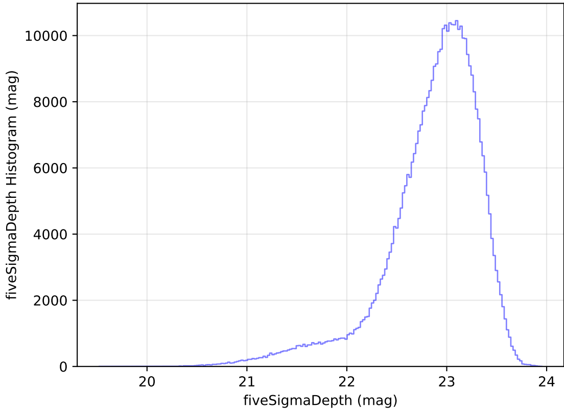
internal_u_expt45_nscale0.9v3.4_10yrs WFD z band: fiveSigmaDepth Histogram
