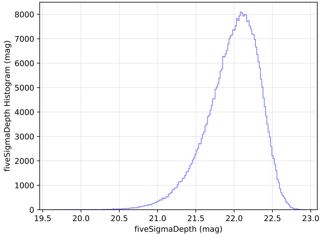
internal_u_expt45_nscale0.9v3.4_10yrs WFD y band: fiveSigmaDepth Histogram
