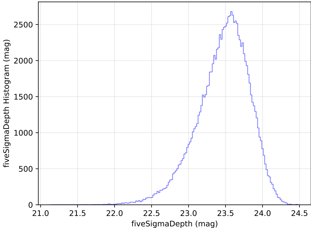
internal_u_expt45_nscale0.9v3.4_10yrs WFD u band: fiveSigmaDepth Histogram
