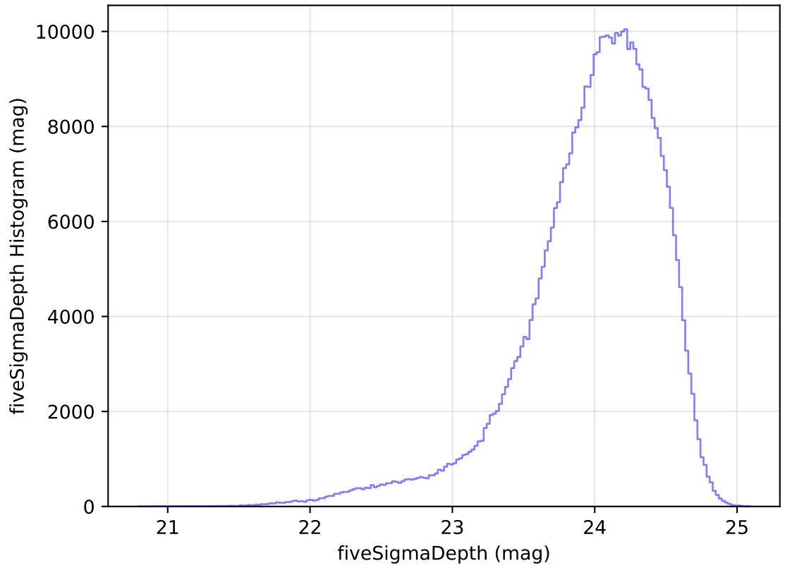
internal_u_expt45_nscale0.9v3.4_10yrs WFD r band: fiveSigmaDepth Histogram
