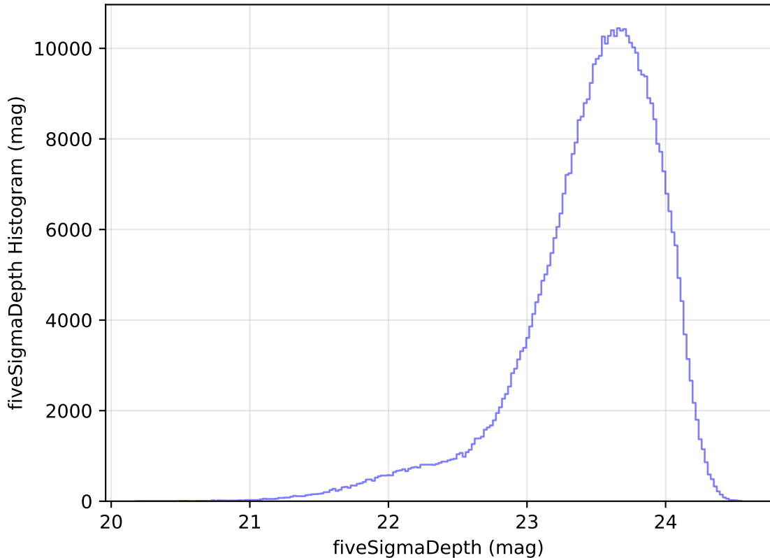
internal_u_expt45_nscale0.9v3.4_10yrs WFD i band: fiveSigmaDepth Histogram
