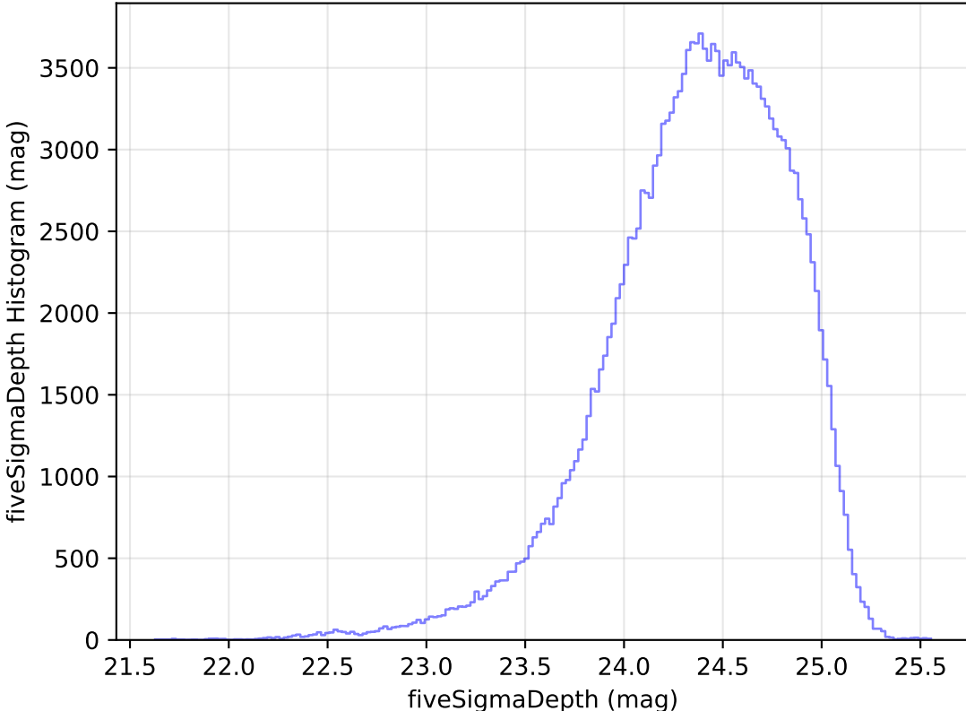
internal_u_expt45_nscale0.9v3.4_10yrs WFD g band: fiveSigmaDepth Histogram
