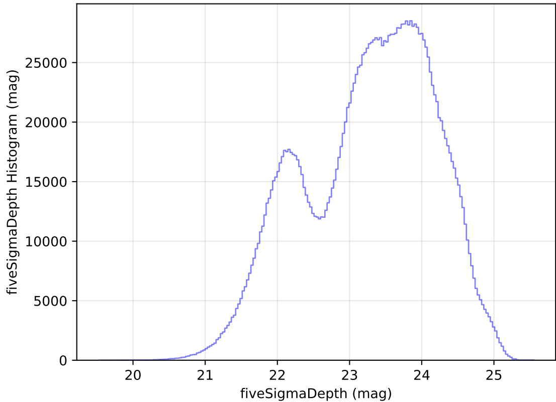
internal_u_expt45_nscale0.9v3.4_10yrs WFD all bands: fiveSigmaDepth Histogram
