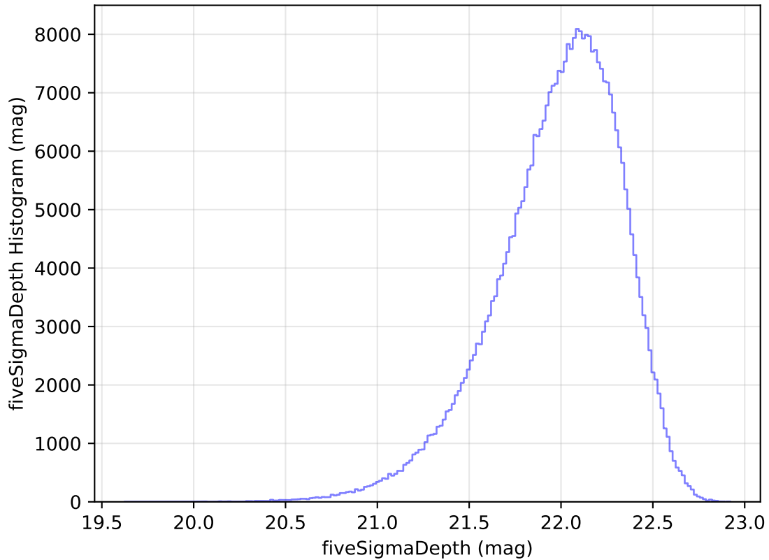
internal_u_expt45_nscale0.9v3.4_10yrs All sky y band: fiveSigmaDepth Histogram
