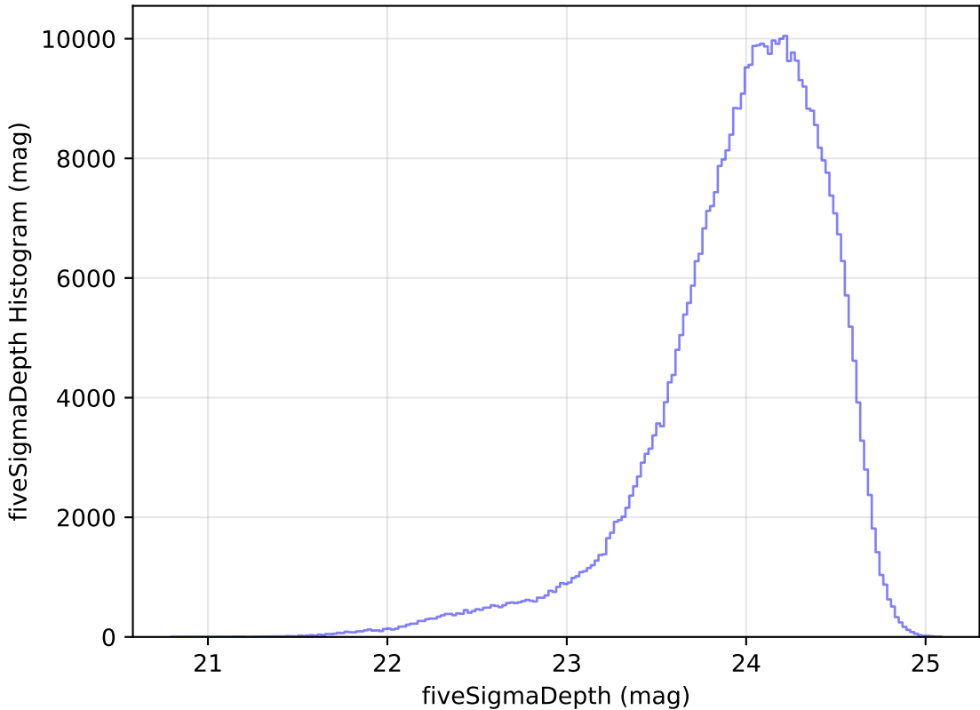
internal_u_expt45_nscale0.9v3.4_10yrs All sky r band: fiveSigmaDepth Histogram
