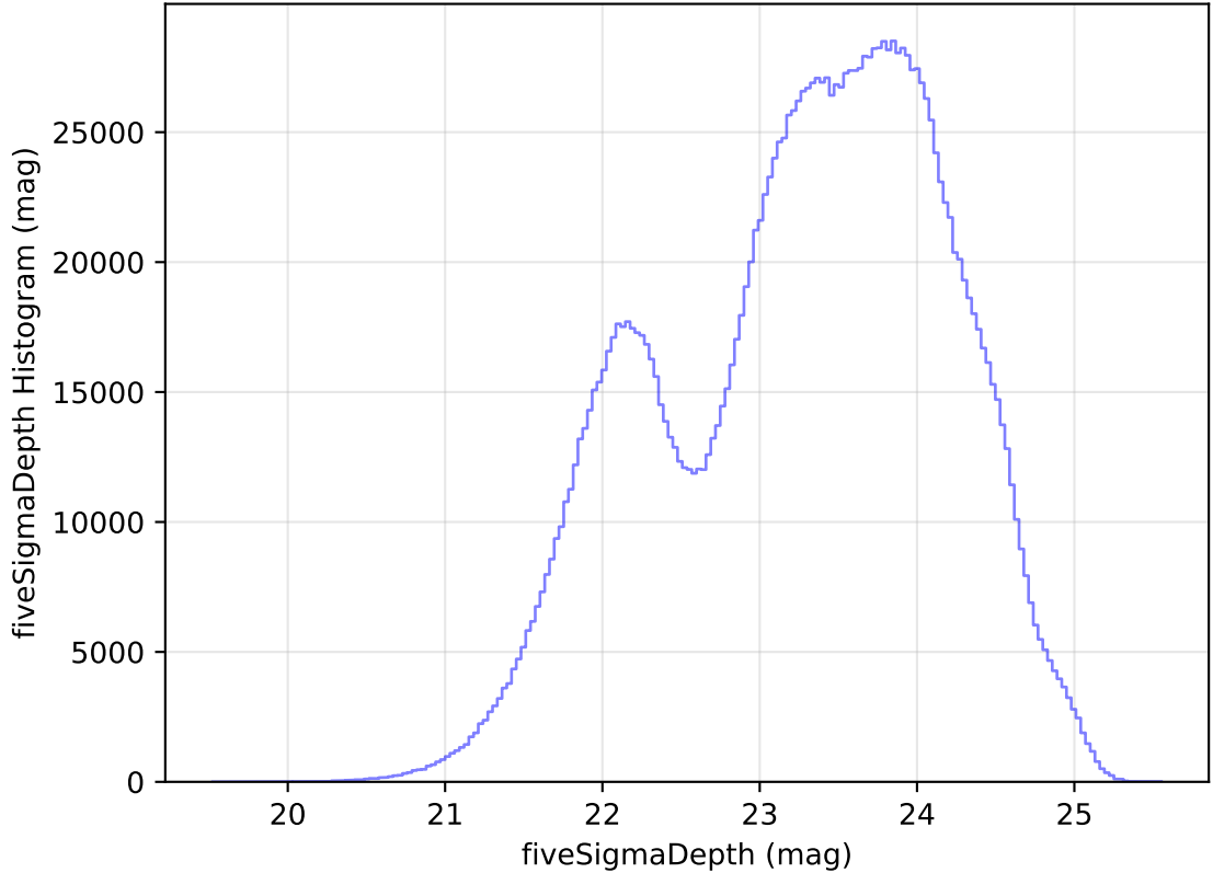
internal_u_expt45_nscale0.9v3.4_10yrs All sky all bands: fiveSigmaDepth Histogram
