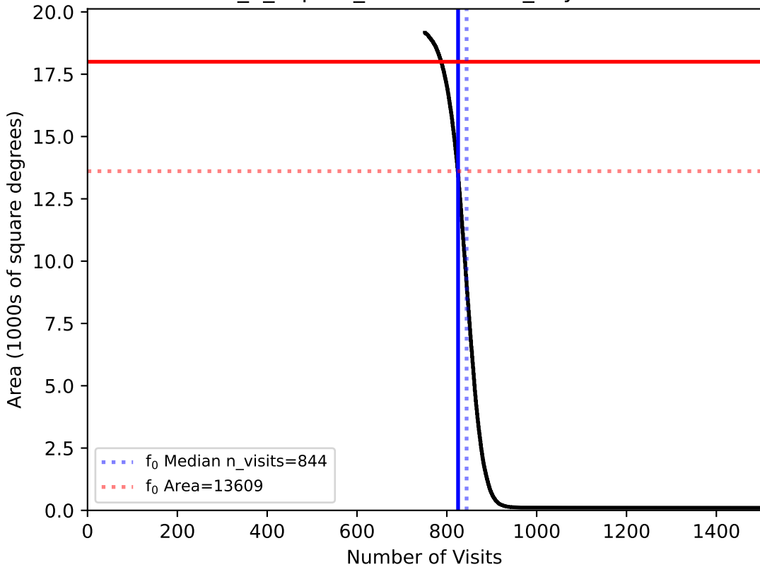
internal_u_expt45_nscale0.9v3.4_10yrs WFD: fO
