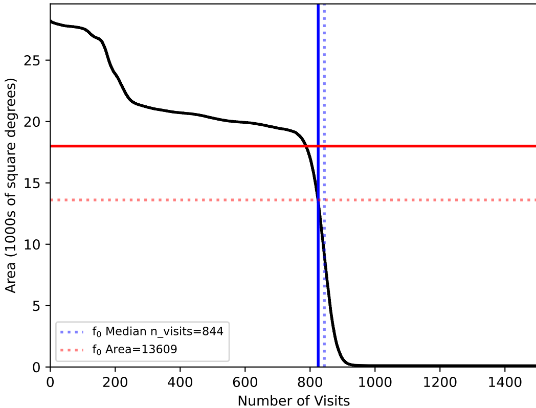
internal_u_expt45_nscale0.9v3.4_10yrs All sky: f0
