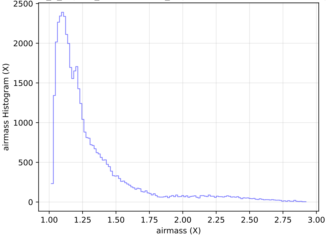
internal_u_expt45_nscale0.9v3.4_10yrs Yr 1 z band: airmass Histogram
