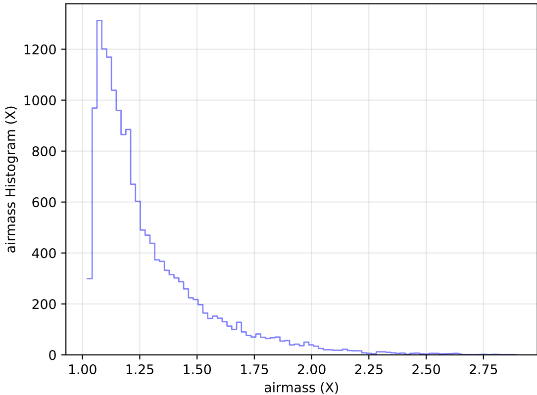
internal_u_expt45_nscale0.9v3.4_10yrs Yr 1 u band: airmass Histogram
