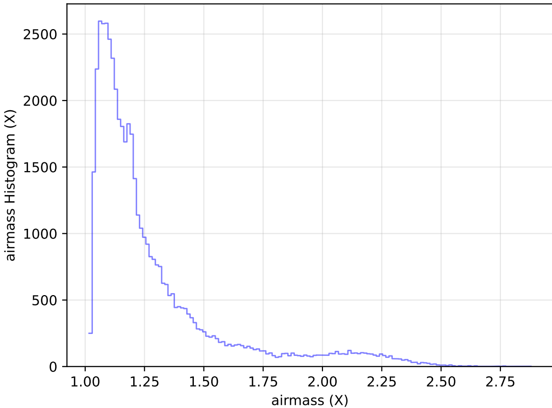
internal_u_expt45_nscale0.9v3.4_10yrs Yr 1 r band: airmass Histogram
