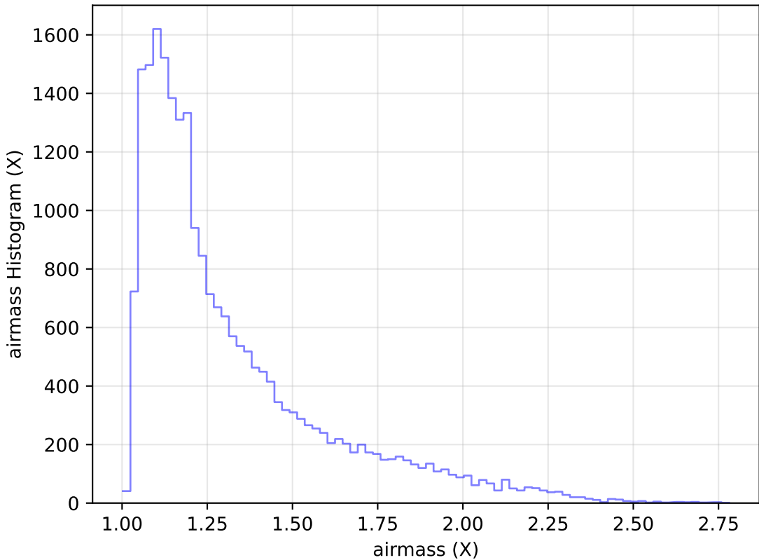
internal_u_expt45_nscale0.9v3.4_10yrs Yr 1 g band: airmass Histogram
