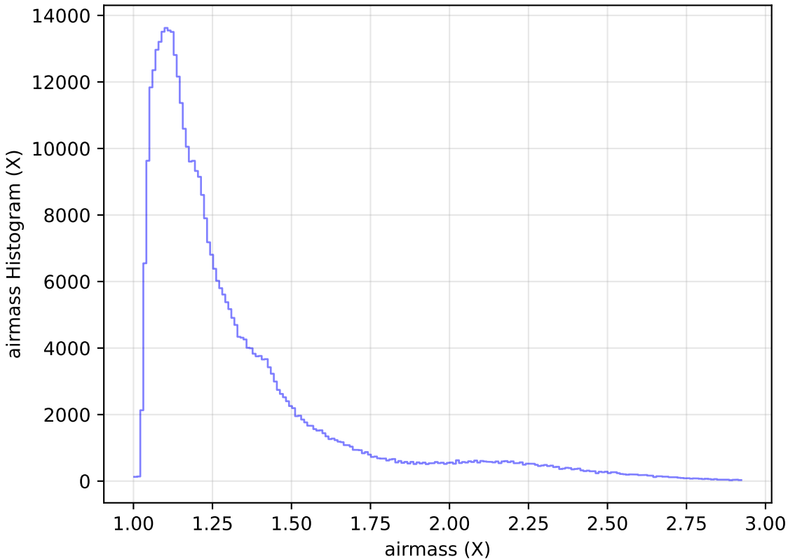
internal_u_expt45_nscale0.9v3.4_10yrs WFD z band: airmass Histogram
