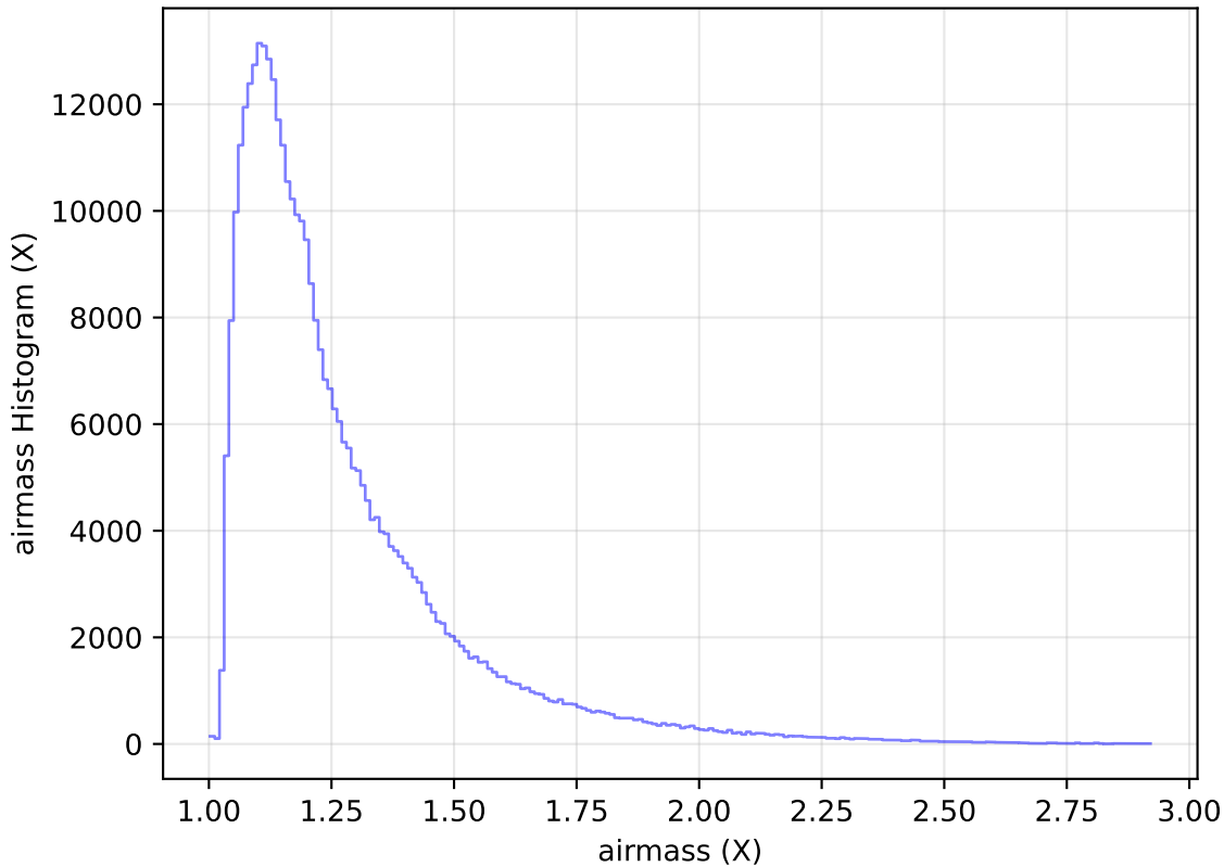
internal_u_expt45_nscale0.9v3.4_10yrs WFD y band: airmass Histogram
