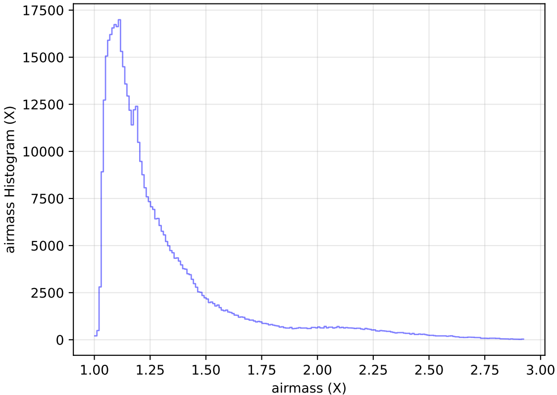
internal_u_expt45_nscale0.9v3.4_10yrs WFD i band: airmass Histogram
