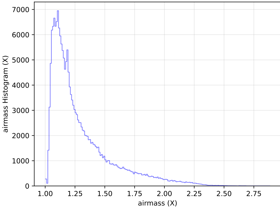
internal_u_expt45_nscale0.9v3.4_10yrs WFD g band: airmass Histogram
