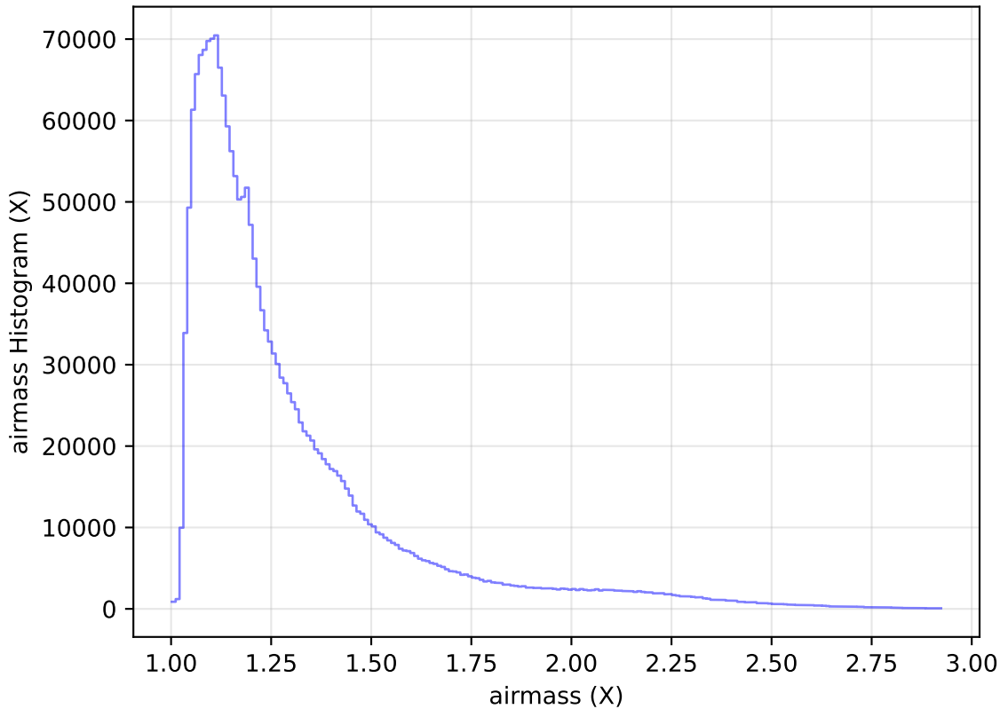
internal_u_expt45_nscale0.9v3.4_10yrs WFD all bands: airmass Histogram
