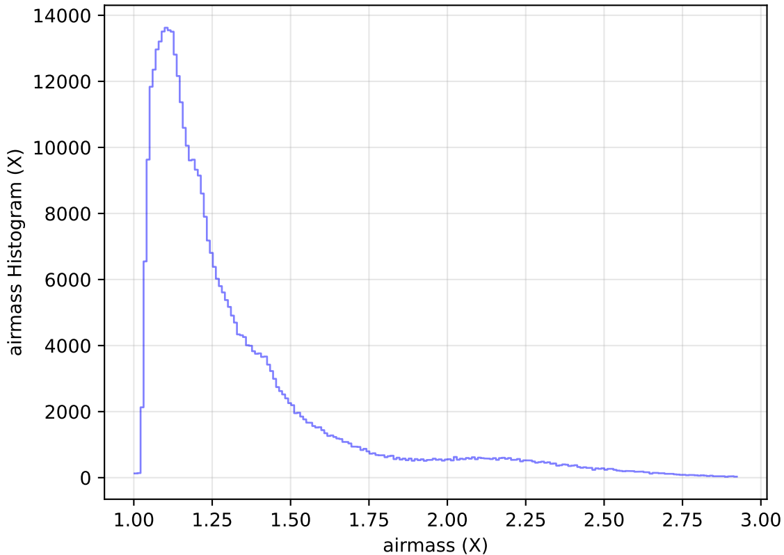
internal_u_expt45_nscale0.9v3.4_10yrs All sky z band: airmass Histogram
