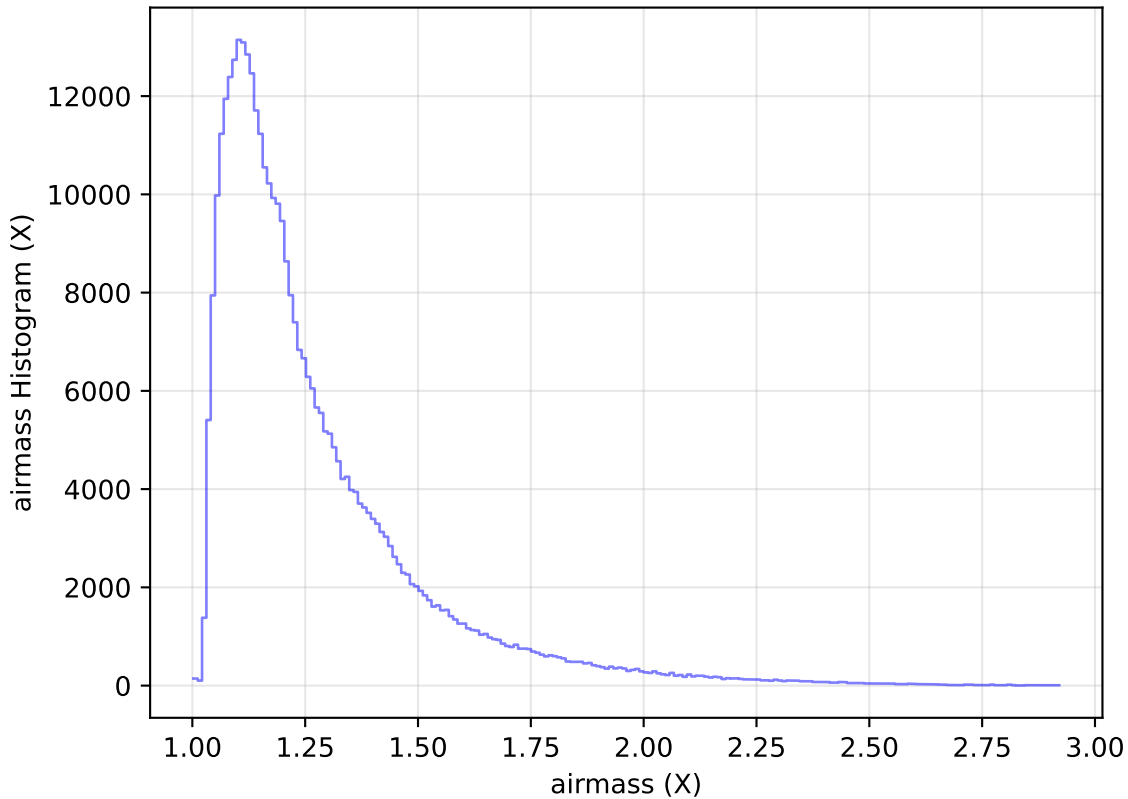
internal_u_expt45_nscale0.9v3.4_10yrs All sky y band: airmass Histogram
