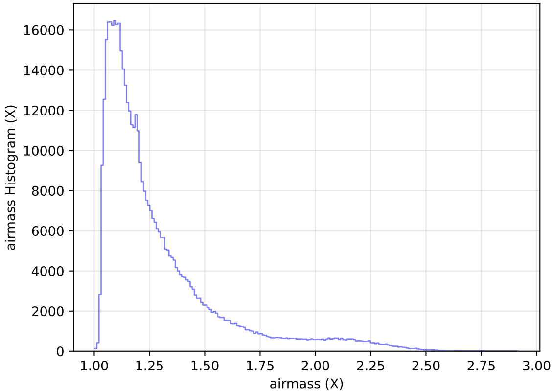
internal_u_expt45_nscale0.9v3.4_10yrs All sky r band: airmass Histogram
