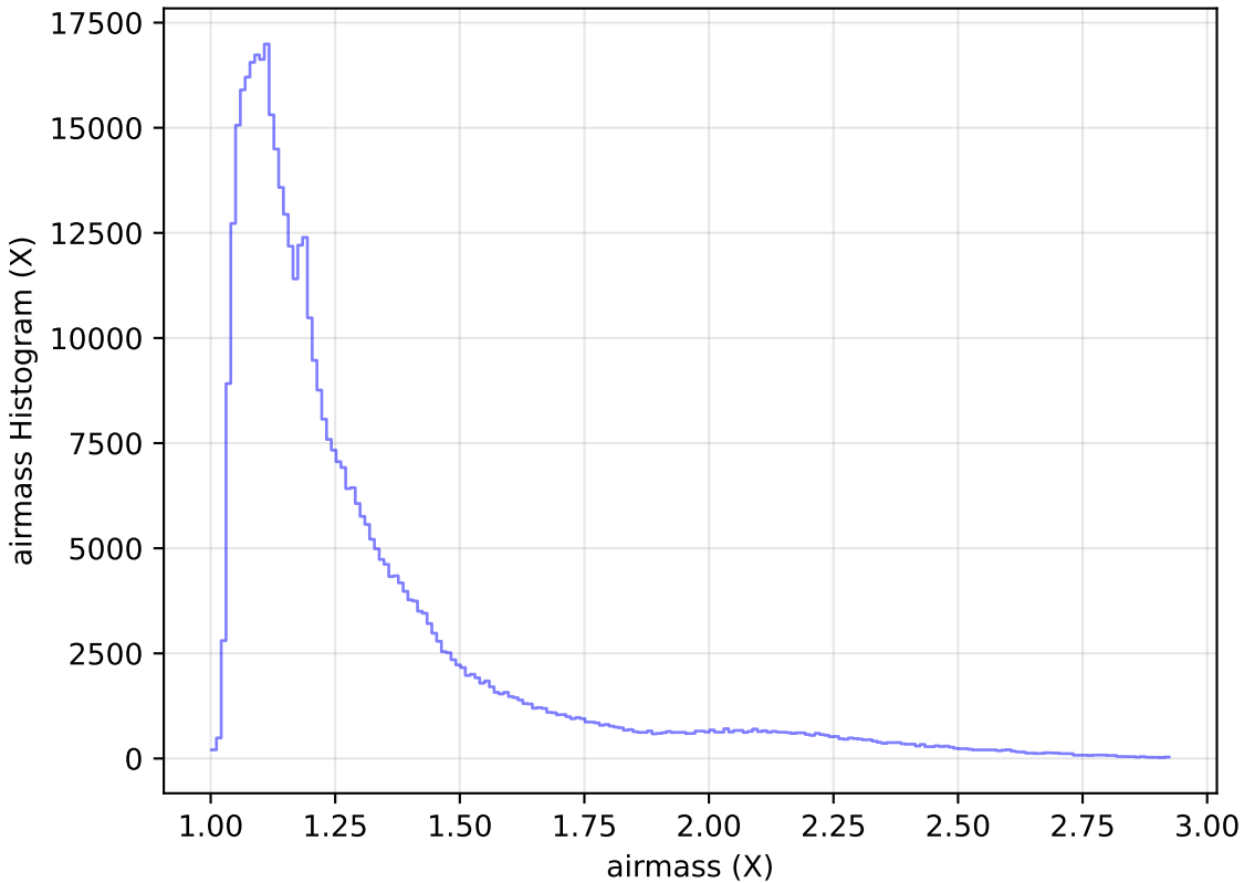
internal_u_expt45_nscale0.9v3.4_10yrs All sky i band: airmass Histogram
