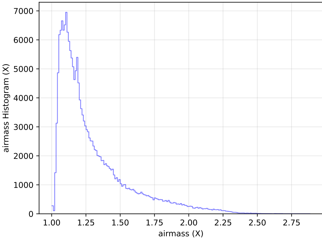
internal_u_expt45_nscale0.9v3.4_10yrs All sky g band: airmass Histogram
