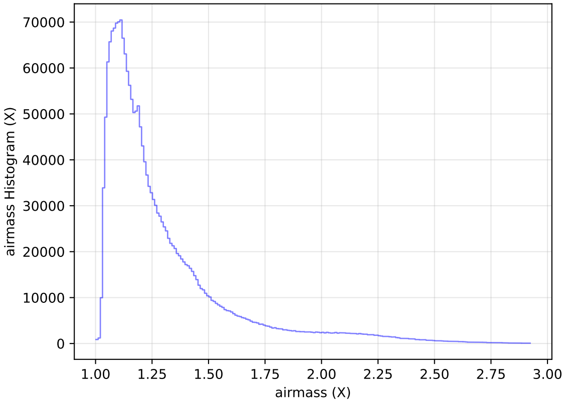
internal_u_expt45_nscale0.9v3.4_10yrs All sky all bands: airmass Histogram
