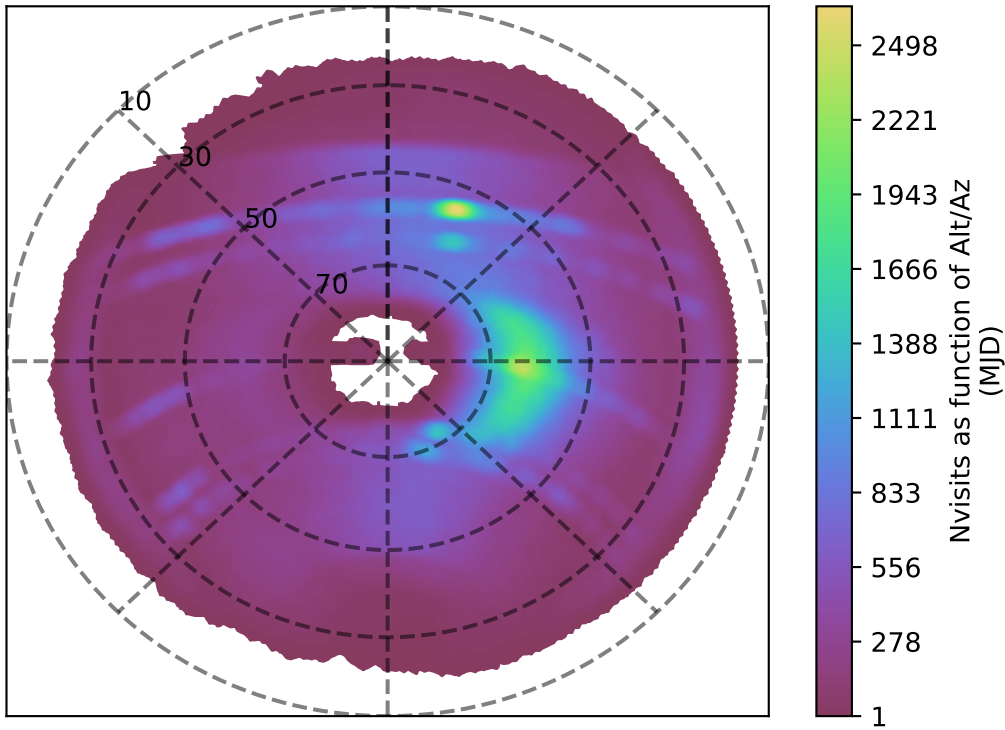
internal_u_expt45_nscale0.9v3.4_10yrs z band: Nvisits as function of Alt/Az
