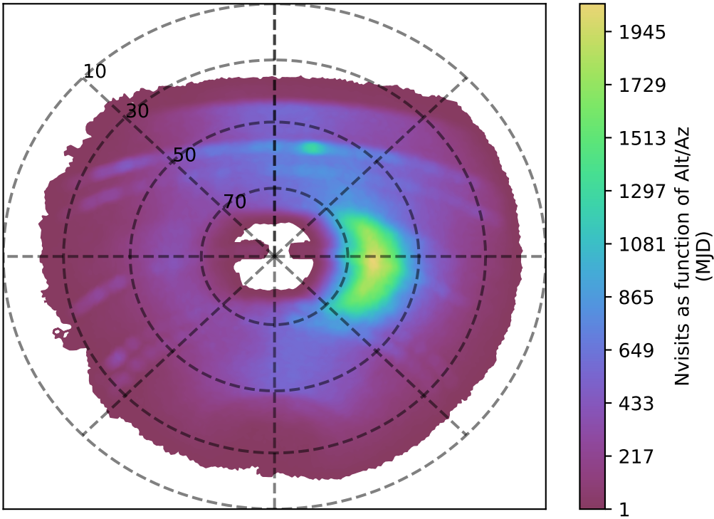
internal_u_expt45_nscale0.9v3.4_10yrs y band: Nvisits as function of Alt/Az
