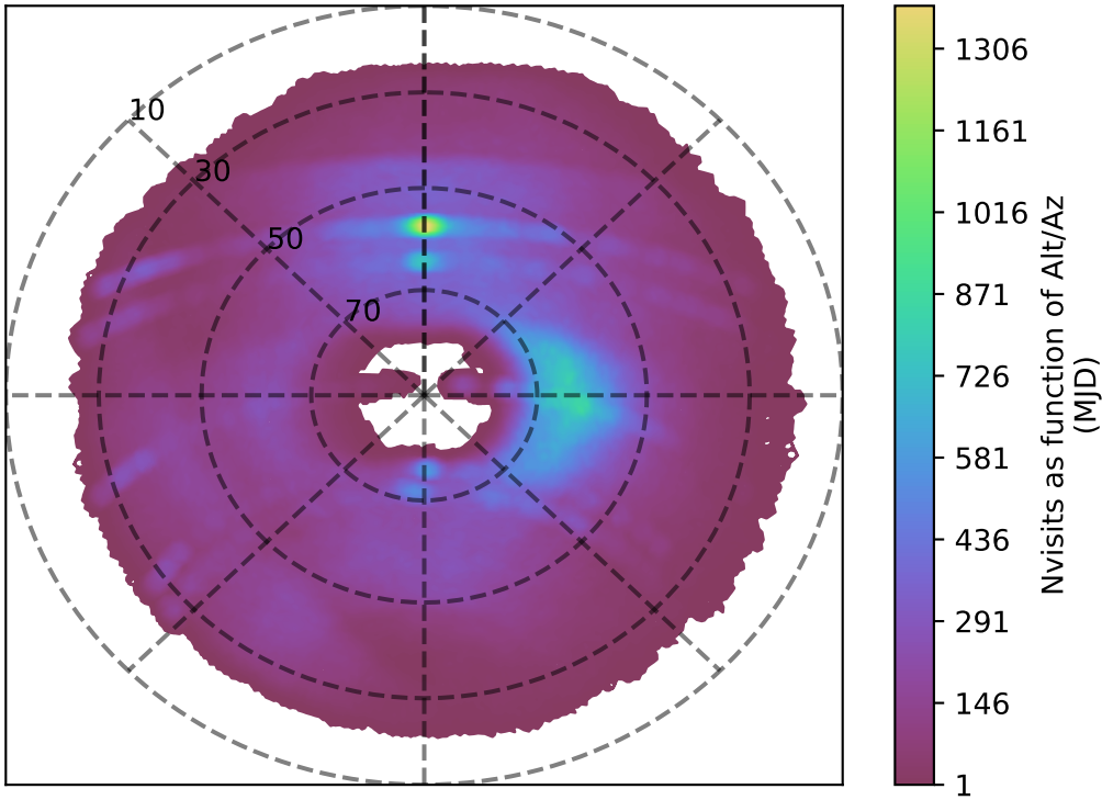
internal_u_expt45_nscale0.9v3.4_10yrs g band: Nvisits as function of Alt/Az
